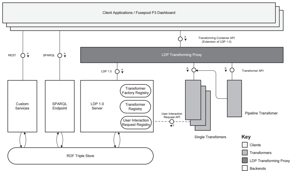
Figure 2: The P3 platform in Fundamental Modeling Concepts (FMC) Notation
