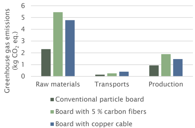
Figure 3: Greenhouse gas emissions in CO 2 -eq. for a conventional particle board, the new developed board with carbon fibers and a conventional particle board with a copper cable.
