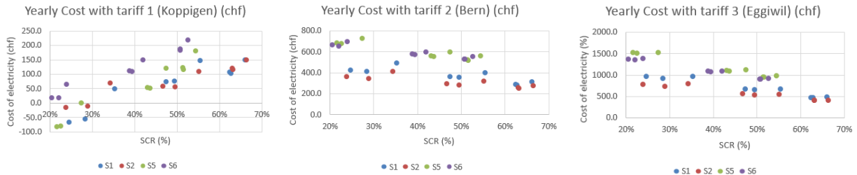
Fig. 6: yearly electricity costs for 3 different electricity tariffs and different control strategies for the four scenarios
