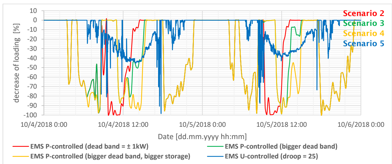
Figure 23: Change of the line loading in percent between the reference scenario and the various configuration of the EMSs
