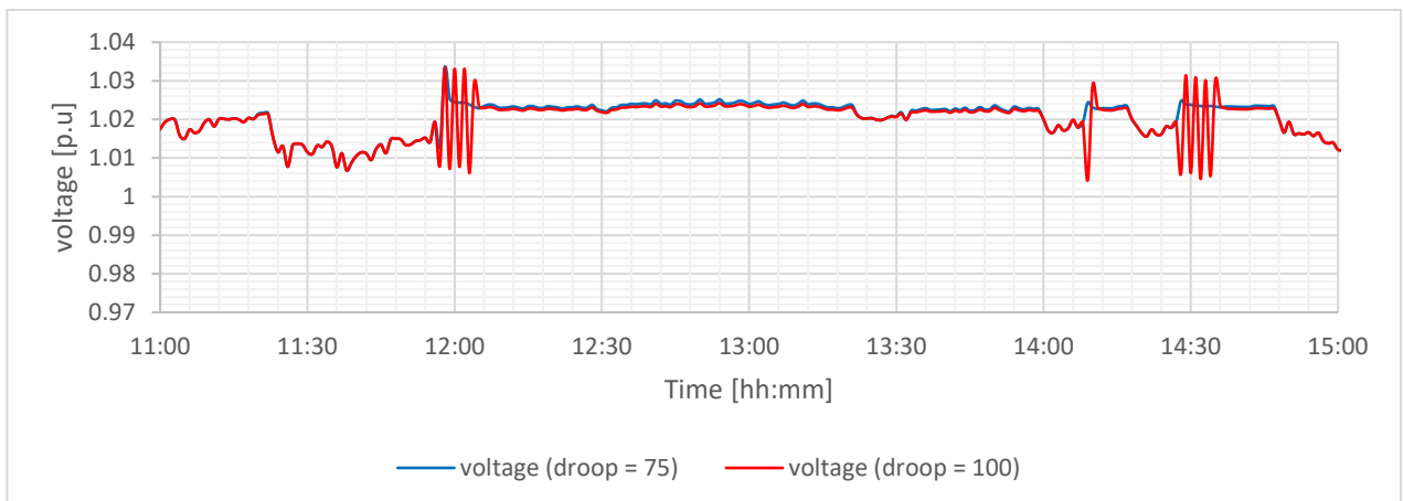
Figure 47: EMS in voltage-controlled mode with a droop value of 75 compared to a droop value of 100
