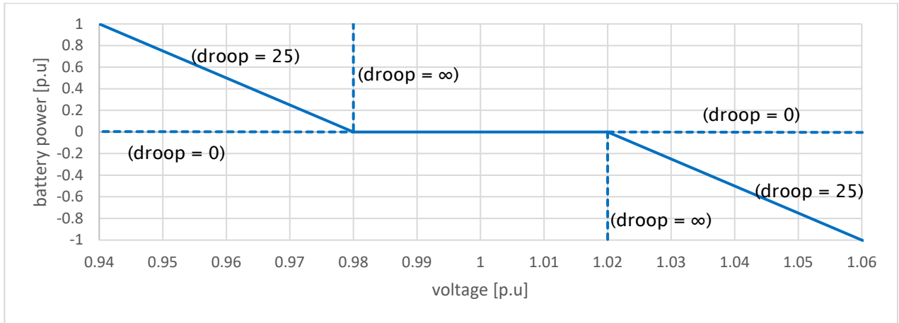
Figure 45: relation between change in voltage and the resulting storage power for different droop values
