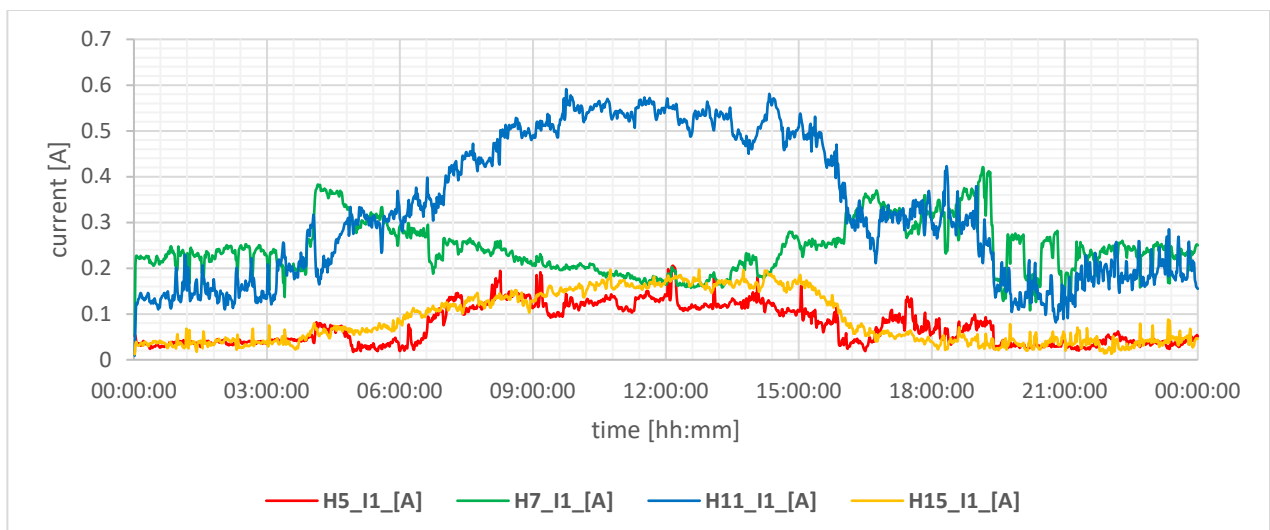
Figure 53: harmonic currents measured after the line model while the Prosumer-Lab was supplied by the house grid and not the grid emulator
