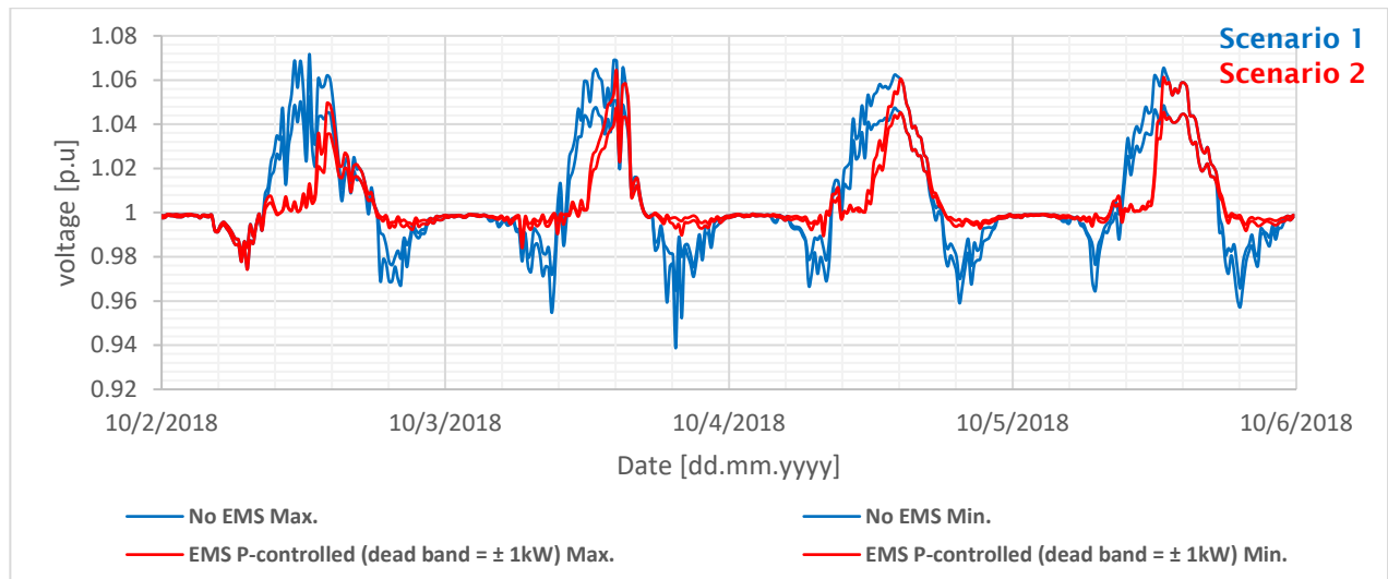
Figure 11: Envelope of the voltages of all simulated grid points
