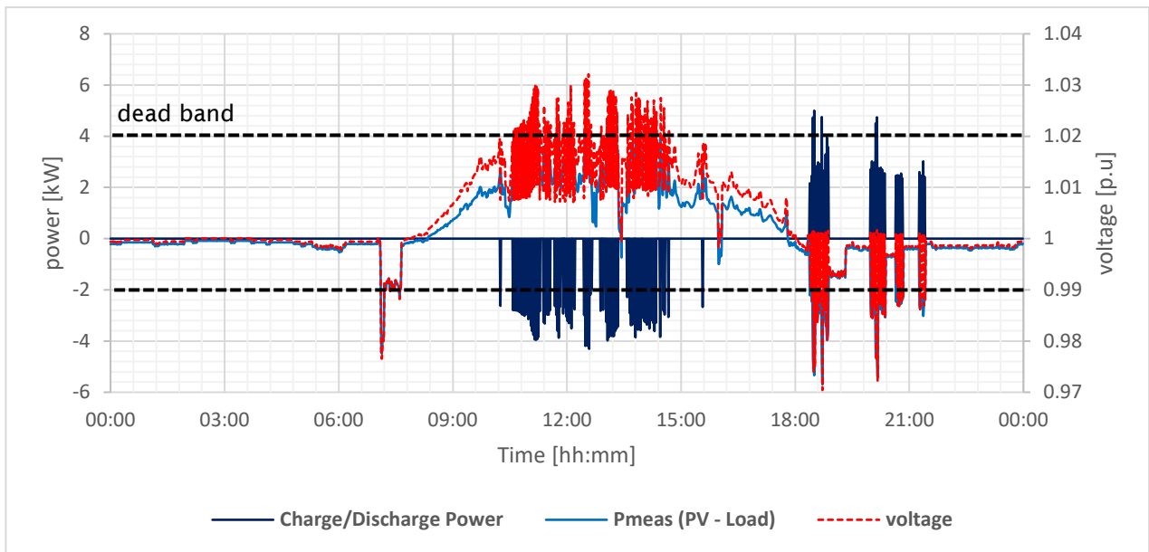
Figure 44: EMS in voltage-controlled mode with no droop value assigned
